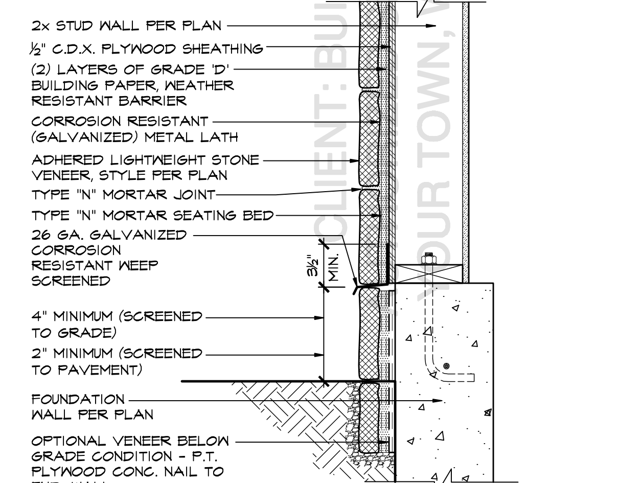
20 ADHERED LIGHTWEIGHT VENEER SCALE: 1 1/2" = 1'-0"
