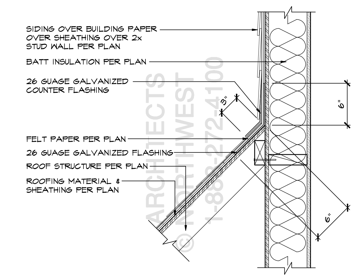
18 ROOF TO WALL FLASHING SCALE: 1 1/2" = 1'-0"
