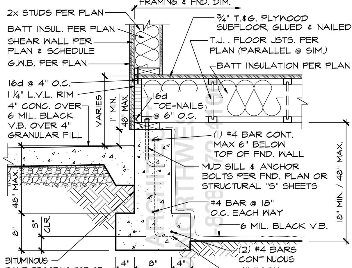
3 8" FND. WALL @ HOUSE/GARAGE SCALE: 1" = 1'-0"
