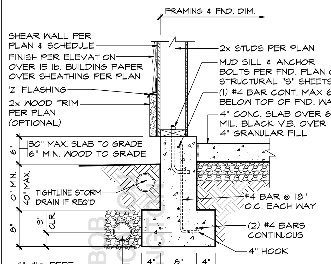
1 8" FND. WALL @ GARAGE SCALE: 1" = 1'-0"
