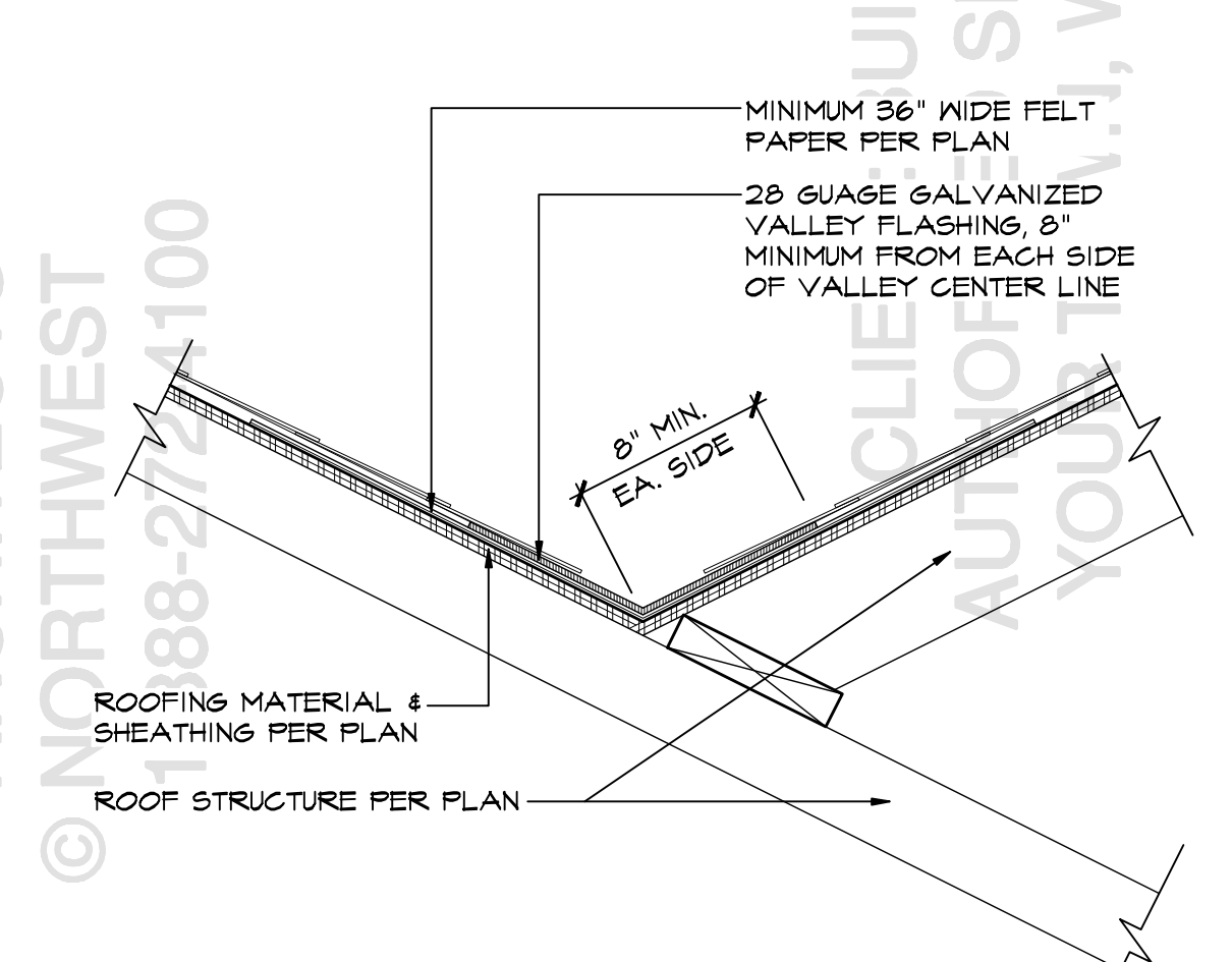
17 ROOF VALLEY FLASHING SCALE: 1 1/2" = 1'-0"
