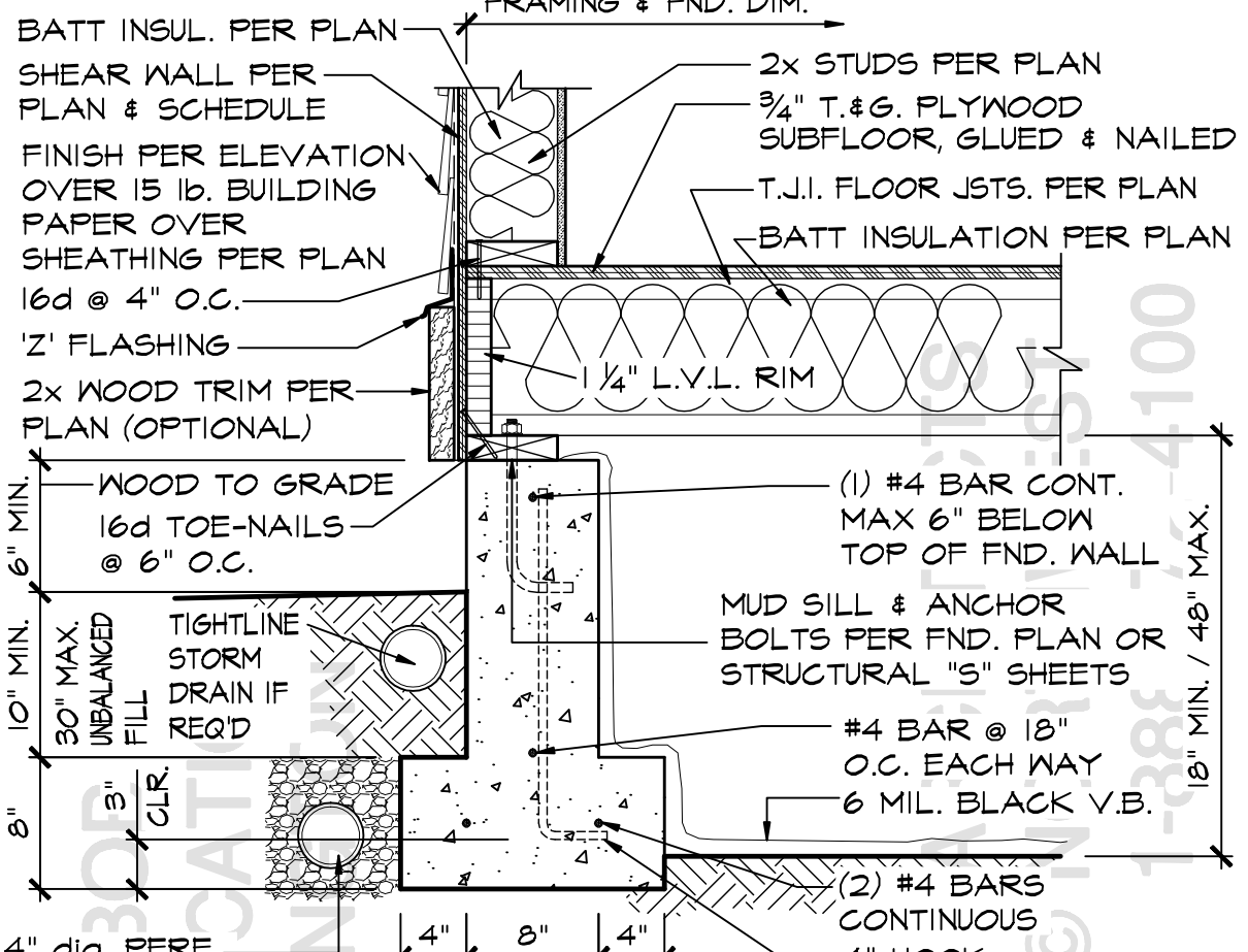
4 TYP. 8" FND. WALL SCALE: 1" = 1'-0"
