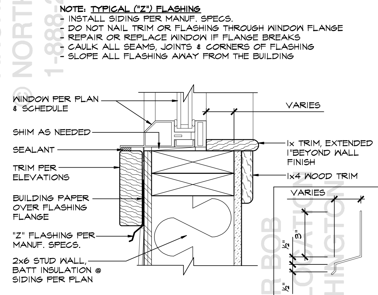
12 TYPICAL WINDOW SILL SCALE: 3" = 1'-0"
