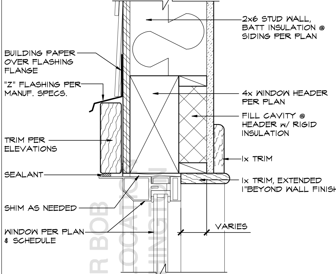
11 TYPICAL WINDOW HEADER SCALE: 3" = 1'-0"
