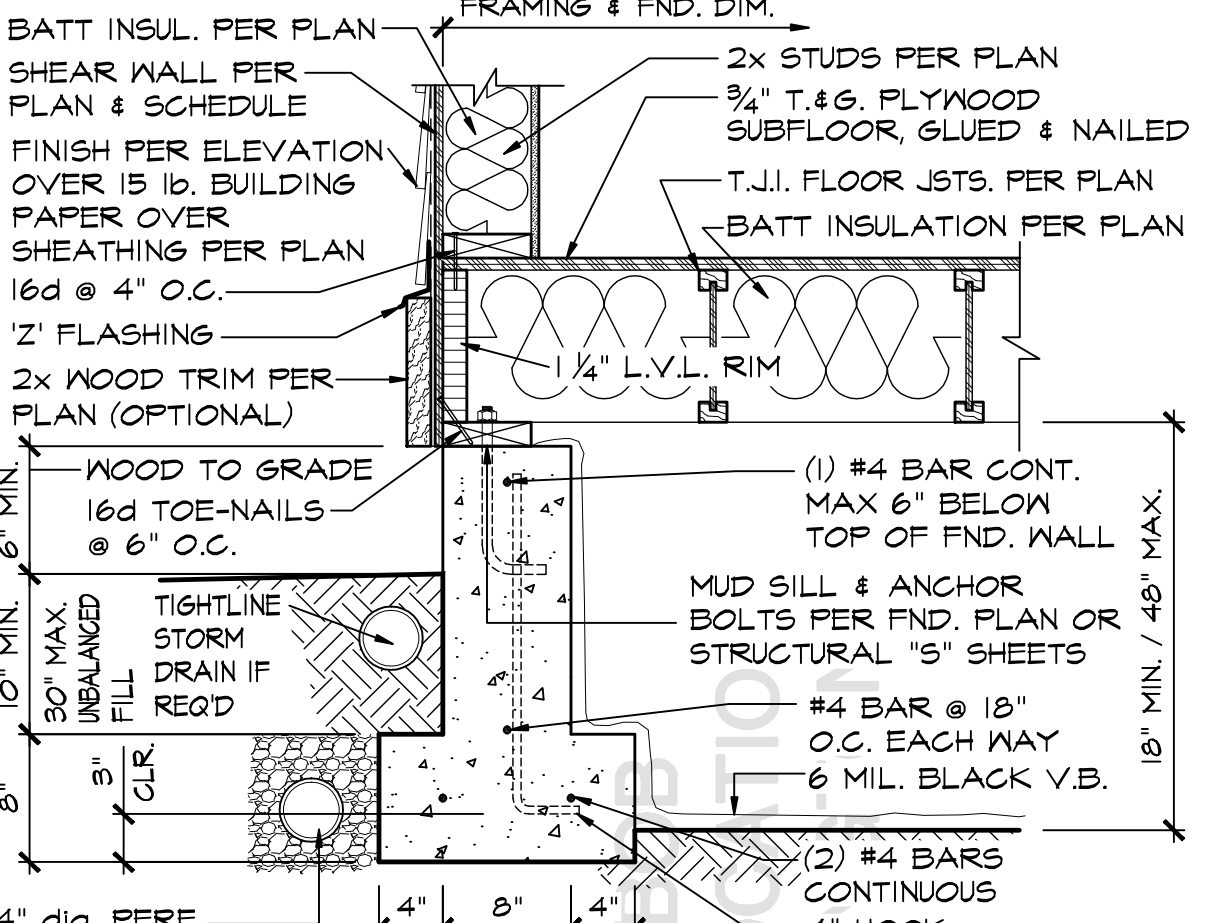
5 TYP. 8" FND. WALL SCALE: 1" = 1'-0"
