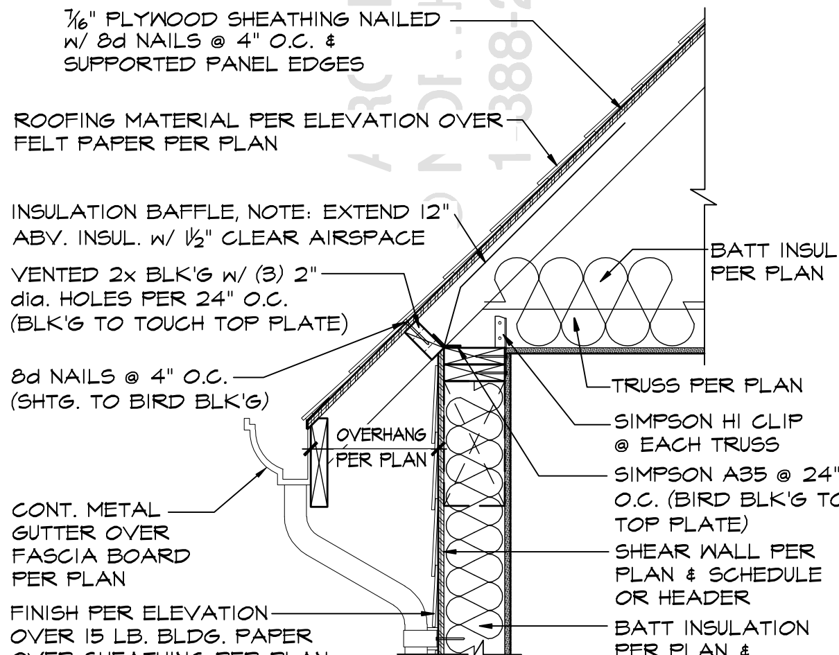
13 FLAT CEILING @ EAVE SCALE: 1" = 1'-0"
