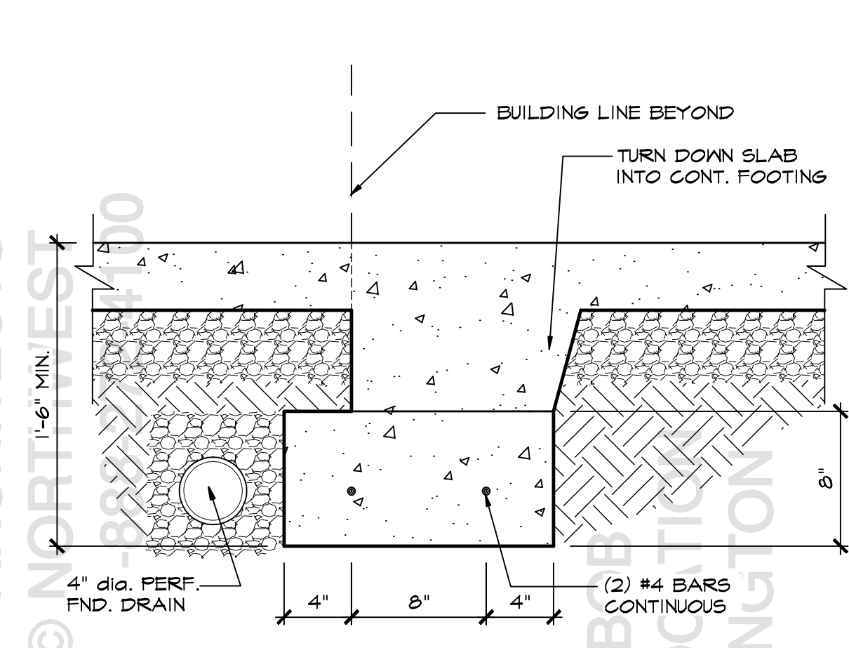
2 THICKENED SLAB @ O.H. DOOR SCALE: 1 1/2" = 1'-0"
