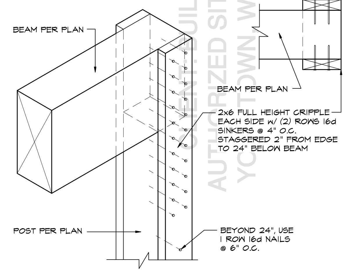
10 BEAM DETAIL SCALE: 1 1/2" = 1'-0"
